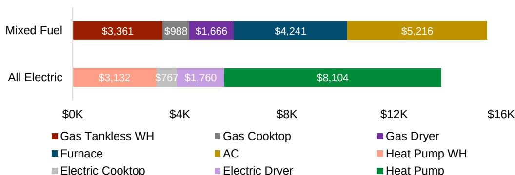
Figure 2-5 Example whole-home capital costs for a single family residential home (new construction, $2021)
