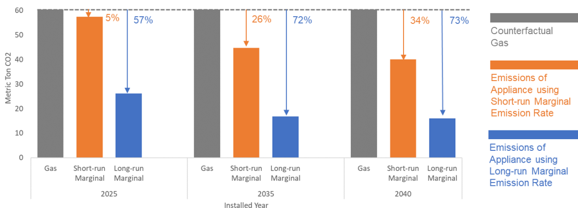
Figure 2-9. GHG Emission Reduction for Single-Family Residential HVAC Electrification, RES
