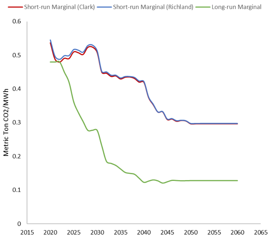
Figure 2-1. Comparison of annual energy sales-weighted short-run marginal greenhouse gas emissions (showing Clark PUD and Richland as examples) from upstream electricity generation versus annual long-run marginal emissions (same across COUs)
