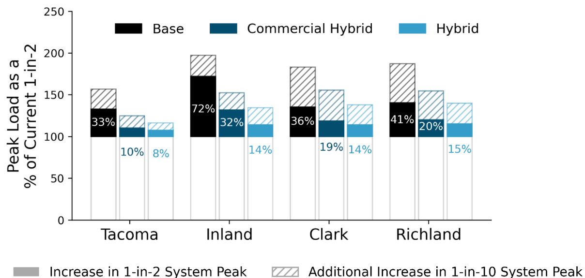
Figure 5-19. Peak Load Growth for Hybrid and Commercial Hybrid Scenarios by 2050
