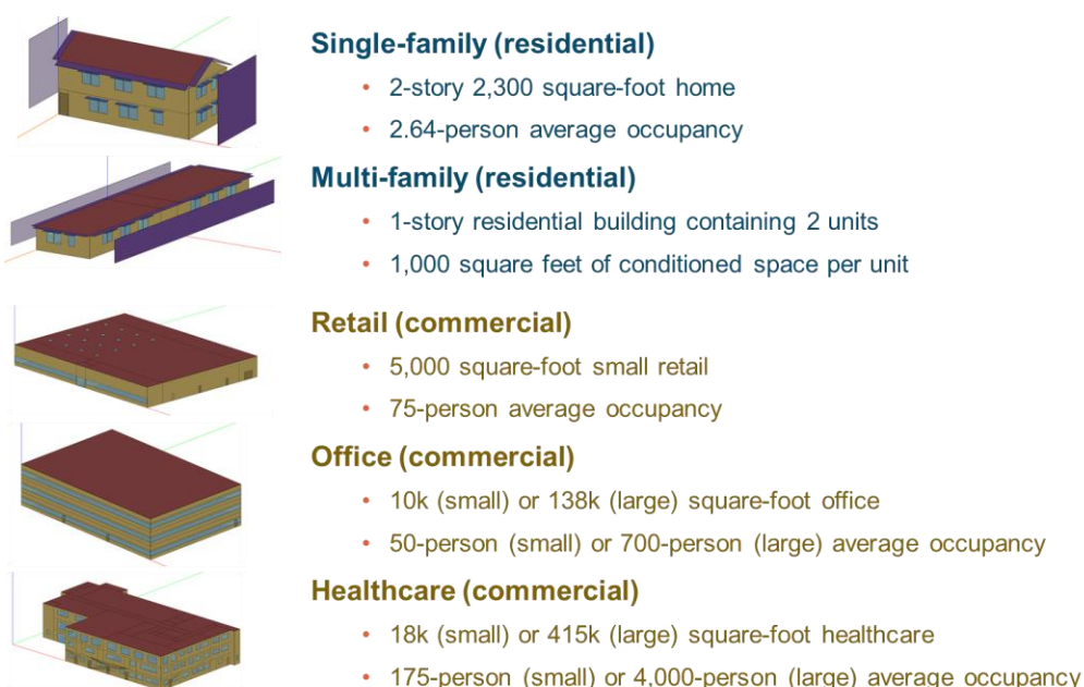
Figure 2-2. Five Building Types Modeled in this Study and Their Characteristics
