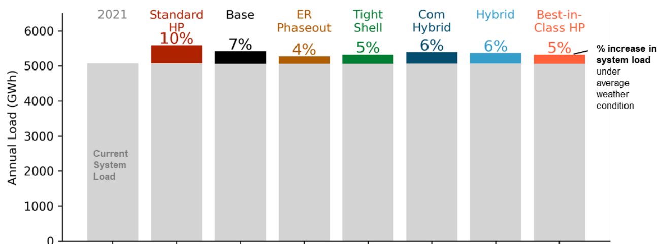
Figure 5-2. Tacoma Power Annual energy sales Growth in 2050
