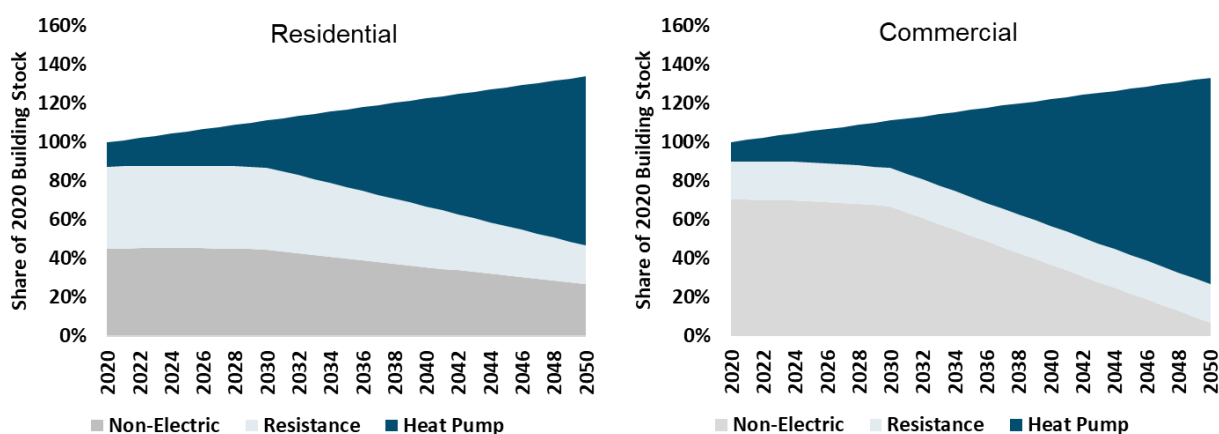
Figure 3-2 Statewide space heating technology mix modeled
