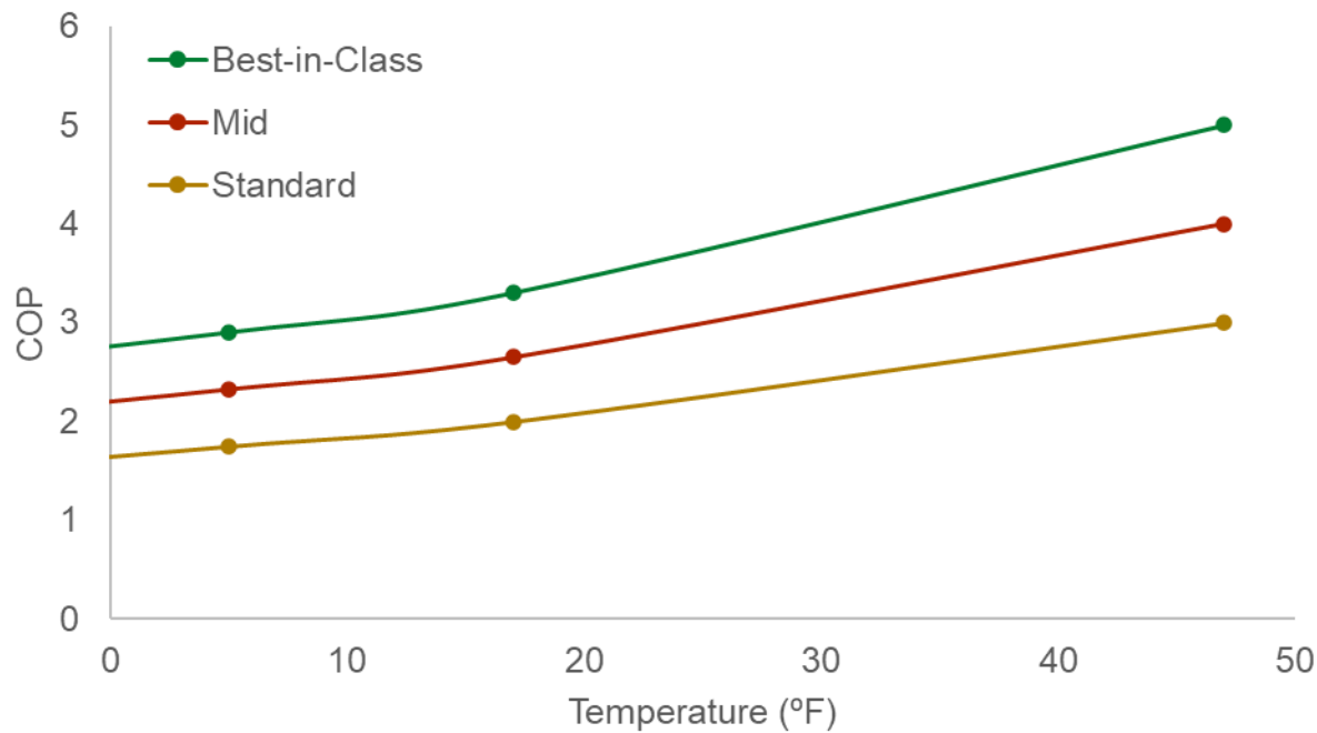
Figure 5-1. RESHAPE COP Curves
