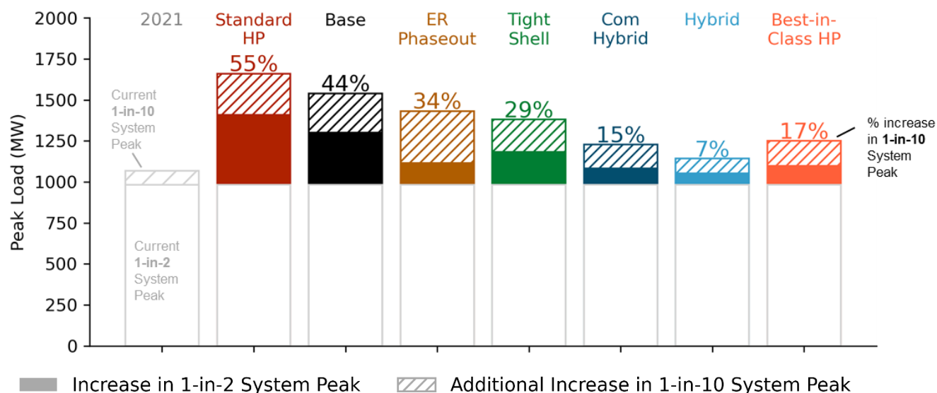
Figure 5-3. Tacoma Power 1-in-2 System Peak Load Growth in 2050
