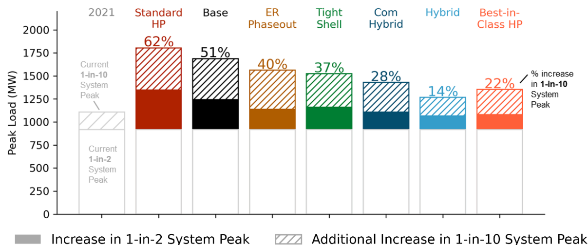
Figure 3-9. Clark PUD 1-in-2 and 1-in-10 Peak Load Growth in 2050 (% growth in 1-in-10 peak load labeled)
