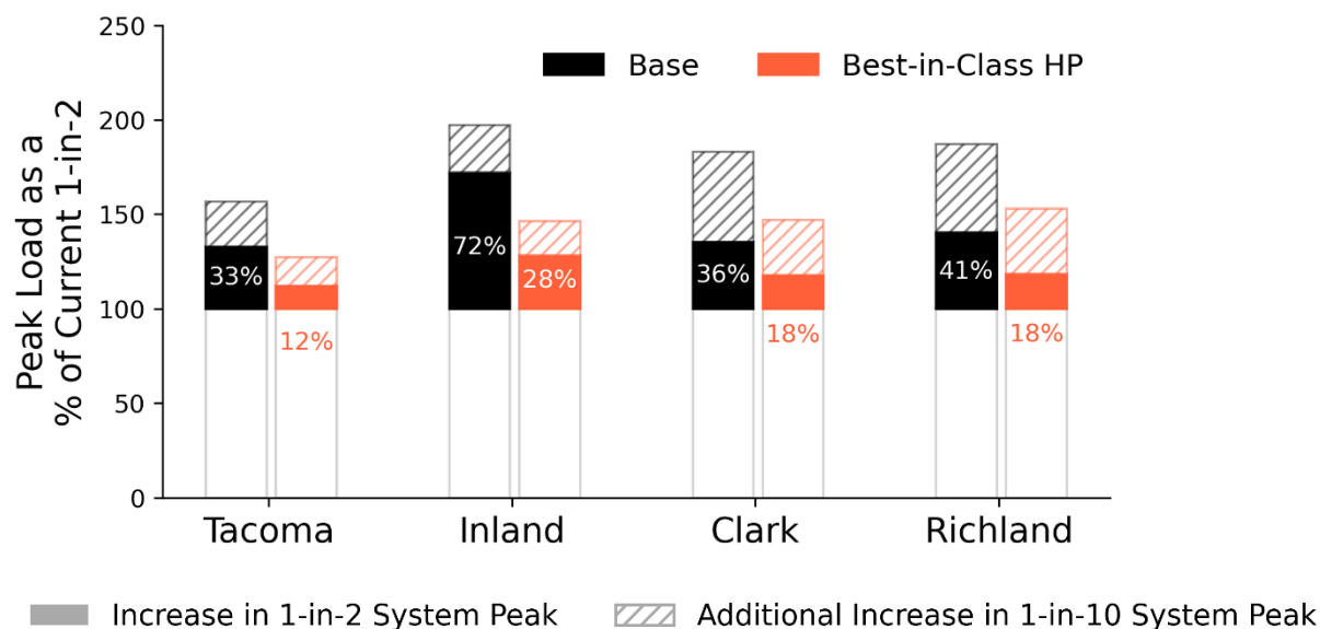
Figure 5-17. Peak Load Growth for Best-in-Class HP by 2050
