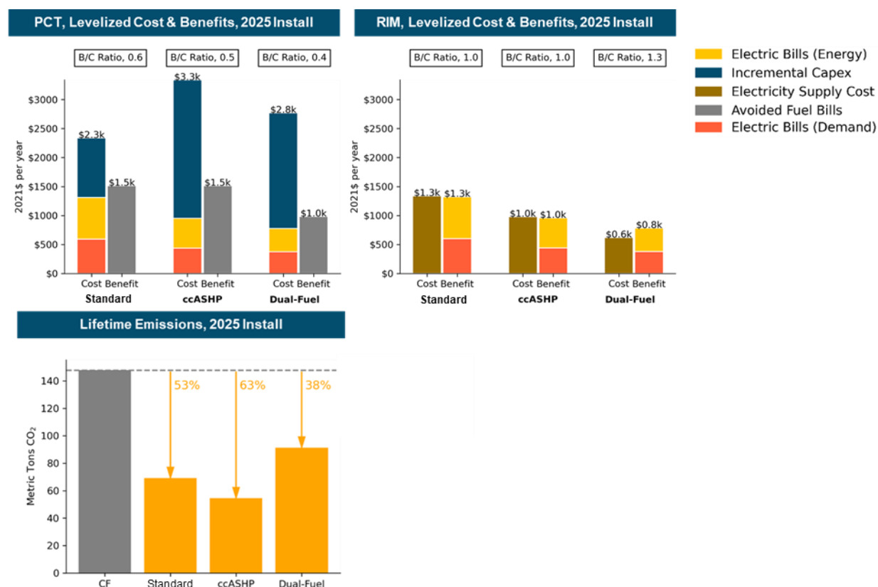
Figure 2-16. Small Retail Retrofit HVAC Electrification, RES
