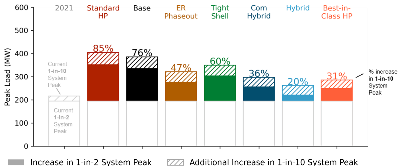
Figure 5-5. IPL 1-in-2 System Peak Load Growth in 2050
