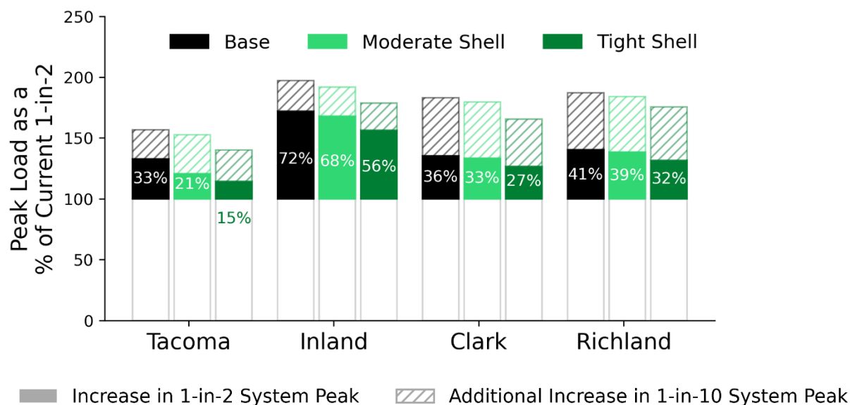
Figure 5-13. Peak Load Growth for Moderate and Tight Shell Scenarios by 2050
