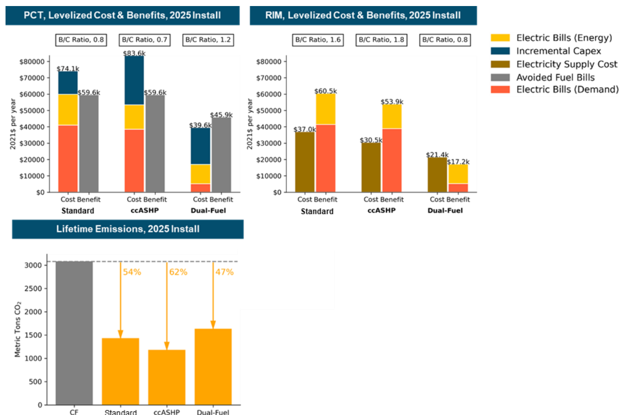
Figure 2-17. Large Office Retrofit HVAC Electrification, Clark PUD
