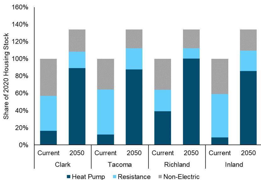
Figure 3-3 Residential Space Heating Technology Mix by COU. Bar charts exceed 100% in 2050 following statewide population growth trends.
