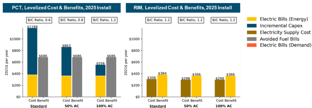
Figure 2-11. Single-Family Residential Retrofit A/C Install Cost Sensitivity, 2025 Installation, Clark PUD
