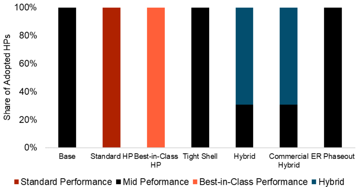
Figure 3-5 Commercial mix of heat pump technology types
