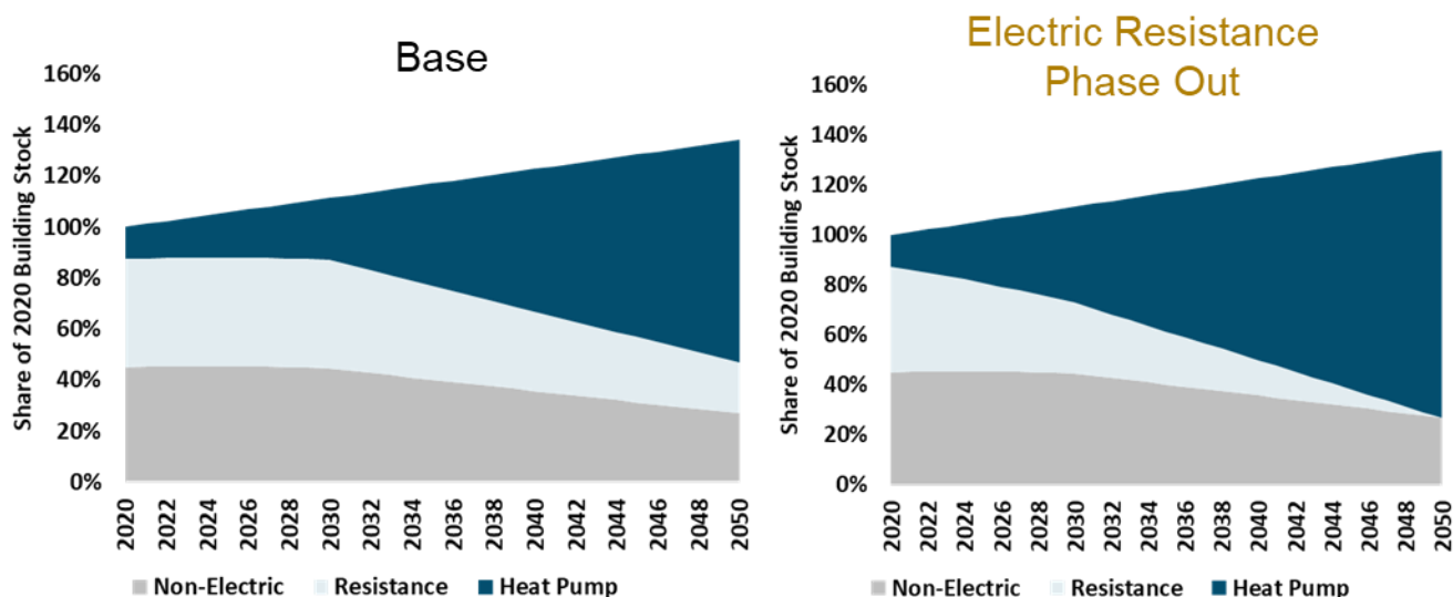
Figure 5-9. Residential building stock comparison in Base and Electric Resistance Phaseout Scenarios
