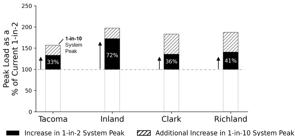
Figure 3-7 Peak Load Growth for Base Case Scenario by 2050
