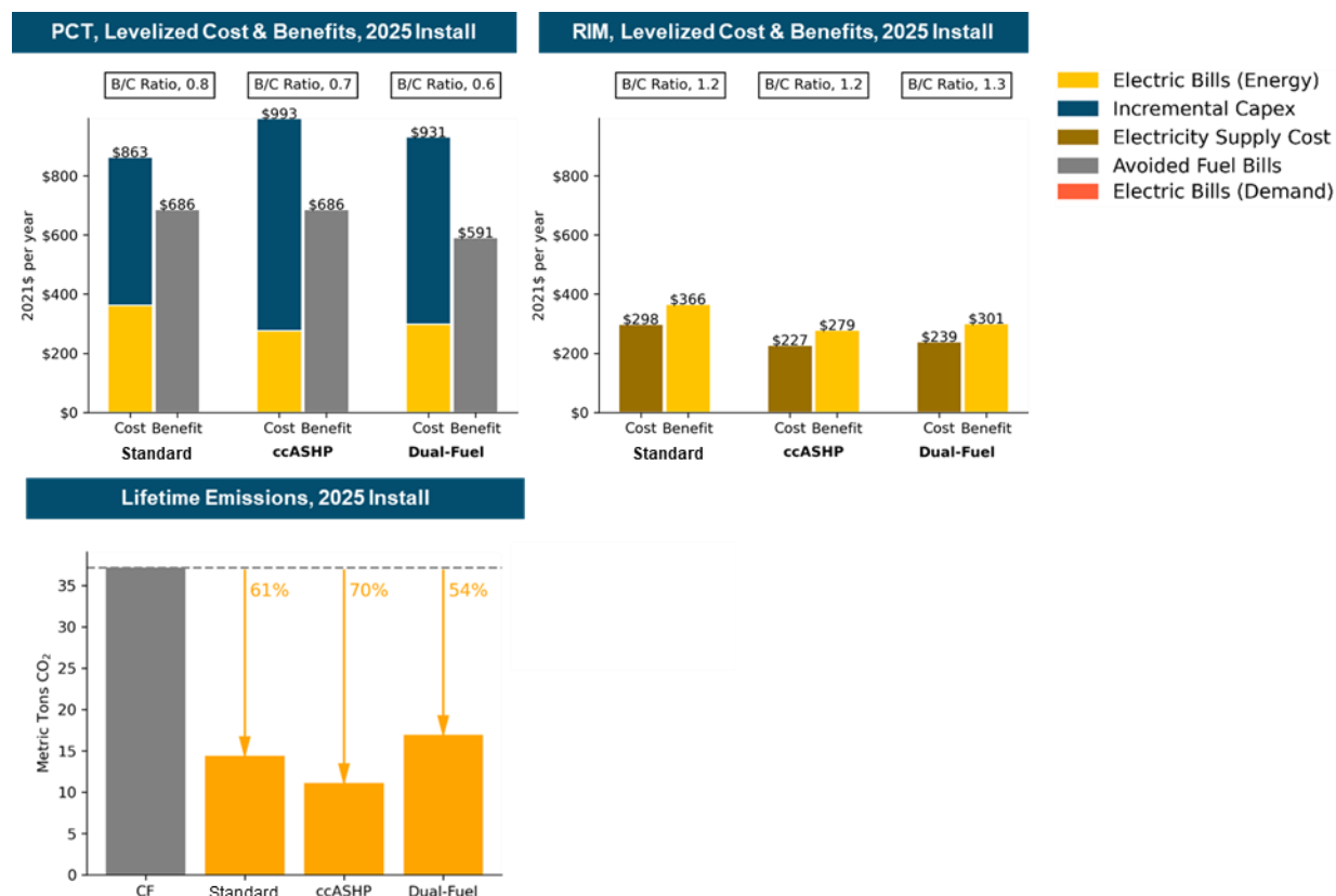
Figure 2-10. Single-Family Residential Retrofit HVAC Electrification, 2025 Installation, Clark PUD
