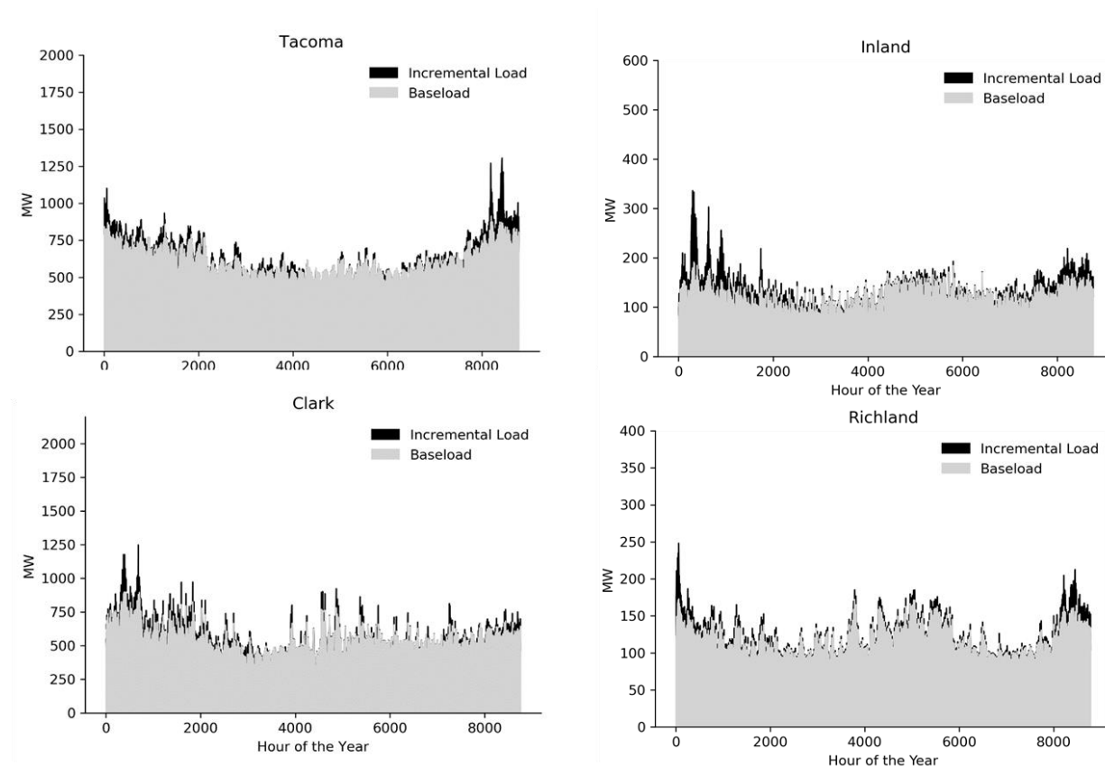
Figure 5-8. Base case scenario system load in 2050 for a 1-in-2 Weather Year (Tacoma: 2016, Inland: 1997, Clark: 2002, Richland: 1984)
