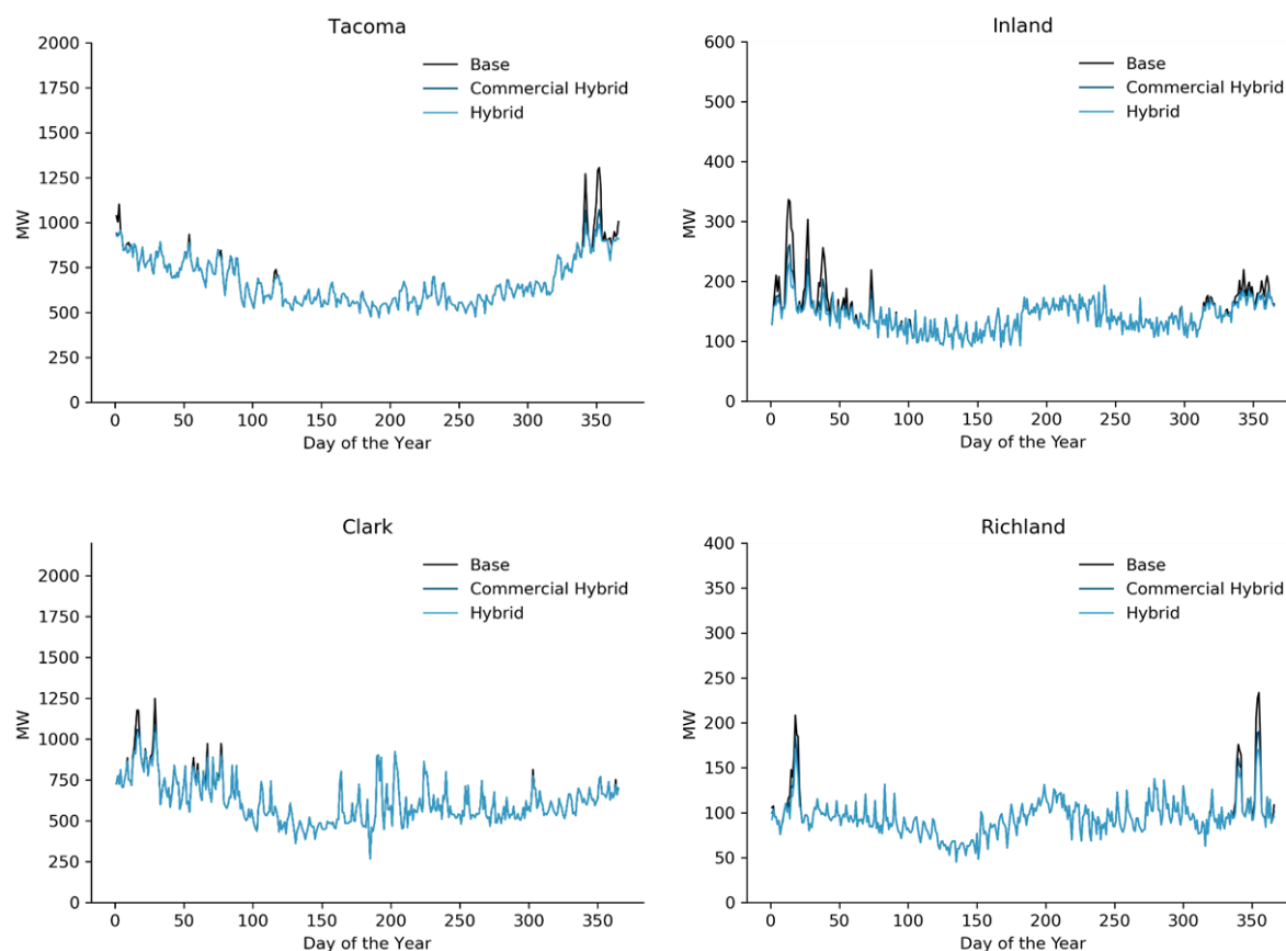
Figure 5-20. Hybrid and Commercial Hybrid scenario system load in 2050 for a 1-in-2 Weather Year (Tacoma: 2016, Inland: 1997, Clark: 2002, Richland: 2016)
