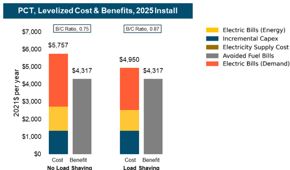
Figure 2-21. Demand Response Sensitivity, Small Office Retrofit Full Building Electrification, 2025 Installation, Clark PUD
