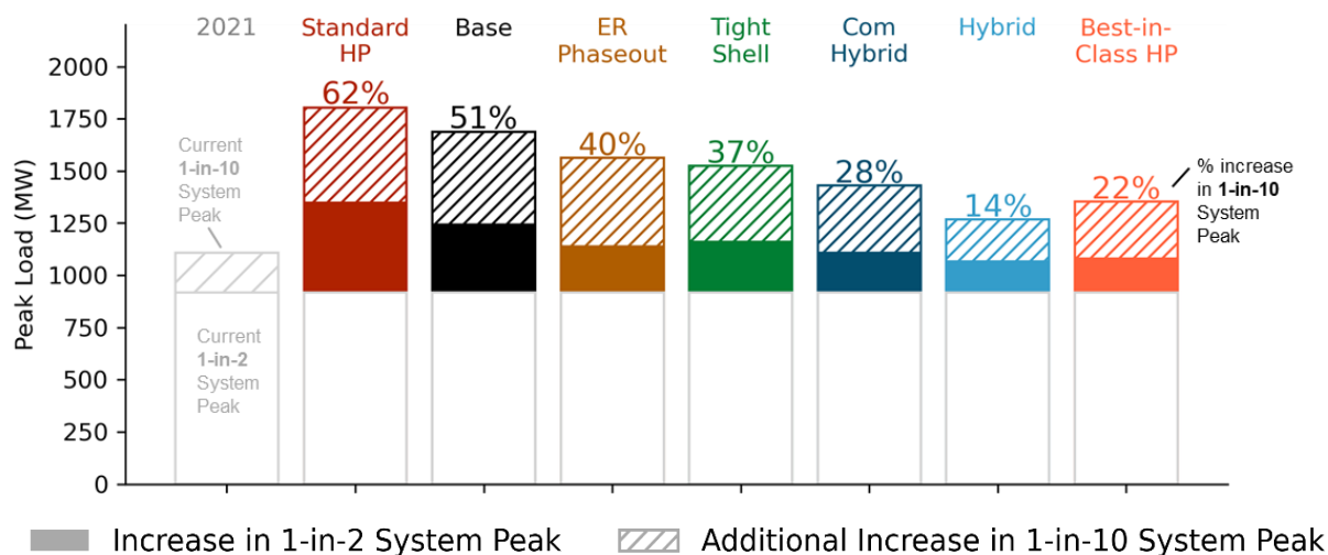
Figure 0-3. Peak Load Growth in 2050 by Scenarios Evaluated in this Study, at the Scales Envisioned in the 2020 Washington State Strategy Study. Results are shown for Clark PUD.
