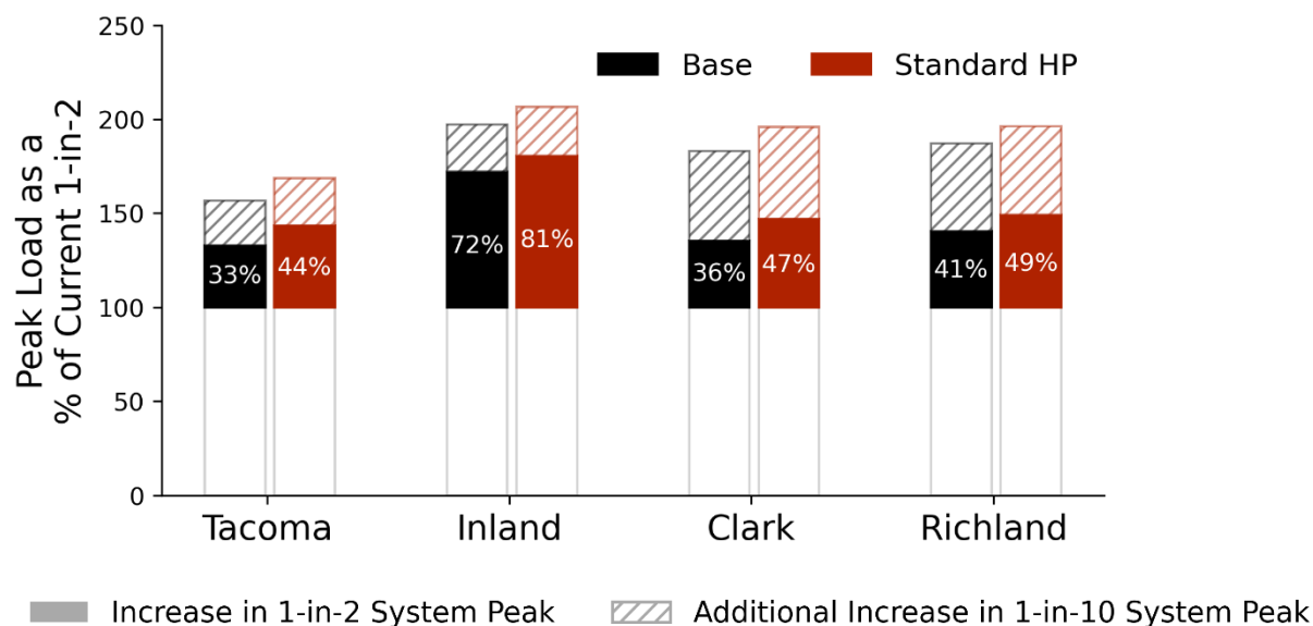
Figure 5-15. Peak Load Growth for Standard HP Scenario by 2050
