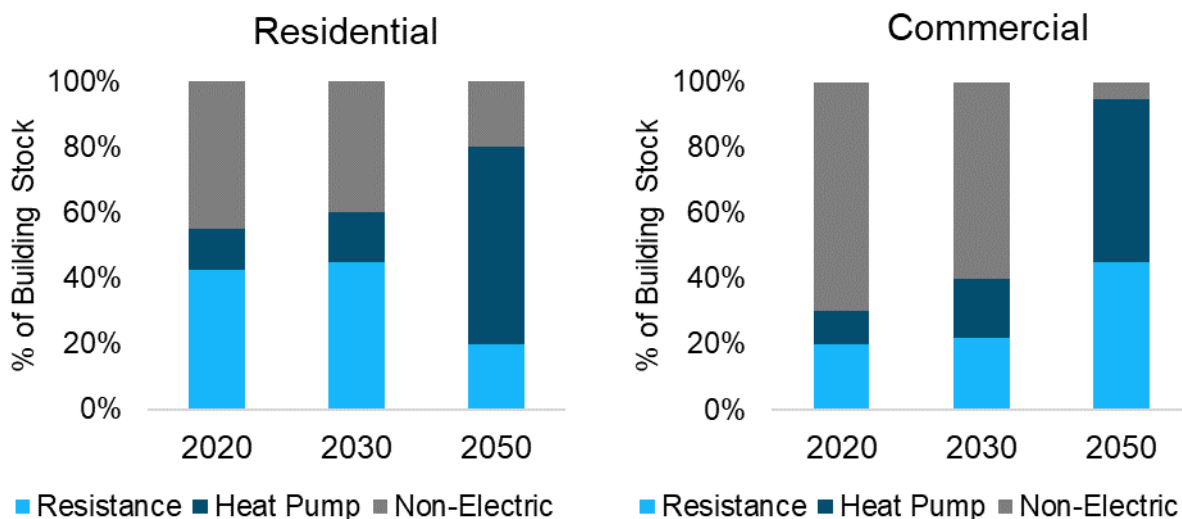
Figure 3-1. 2021 Washington State Energy Strategy Space Heating Technology Mix 22
