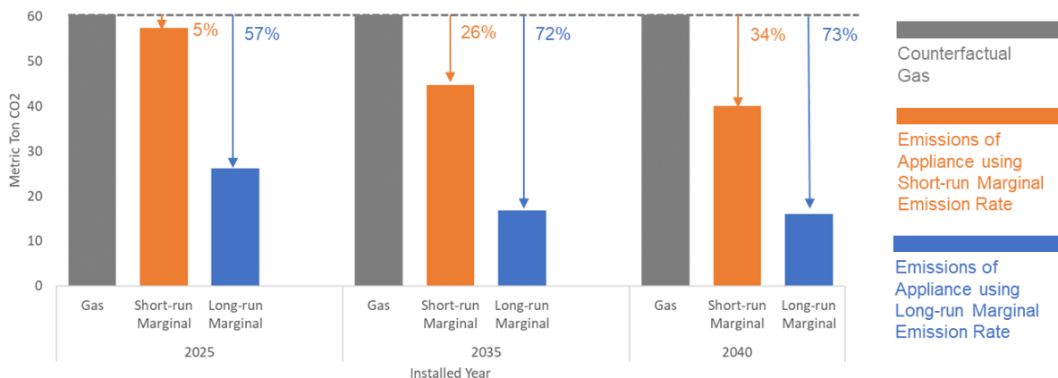
Figure 0-1. Lifetime emissions of a gas furnace vs. a standard heat pump HVAC system in a single-family home in Richland Energy Services' service area.
