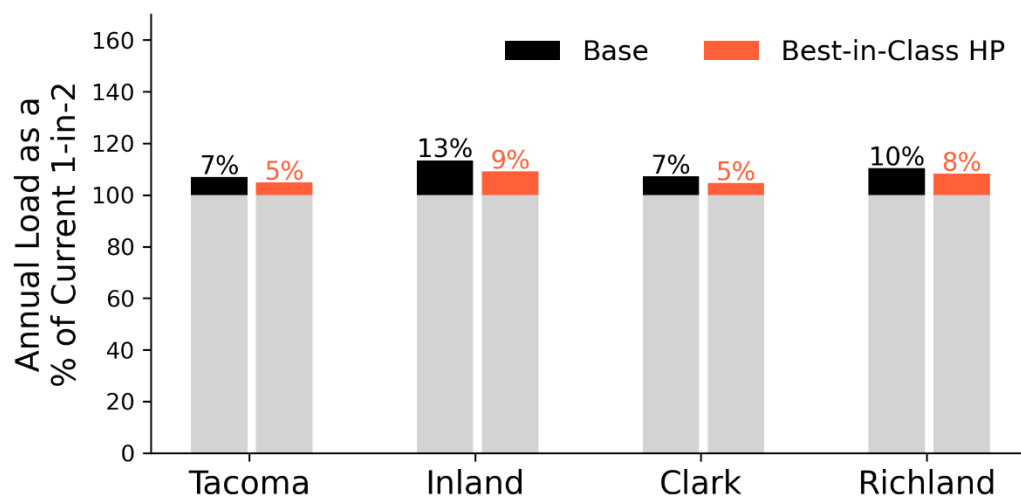
Figure 5-16. Annual energy sales Growth (1-in-2) Best-in-Class Scenario by 2050
